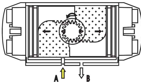
Double Acting Operation Function (Standard Rotation) Top View
