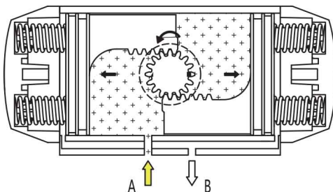
Single Acting Operation Function (Standard Rotation) Top View
