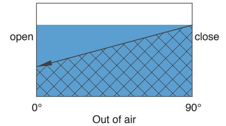
Output Torque of Spring Return Actuator
