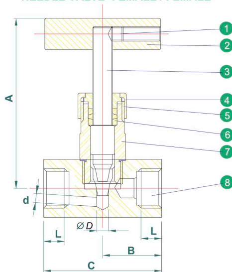
NEEDLE VALVE- FEMALE / FEMALE
